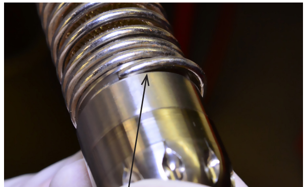
Over-Tightened Spring
