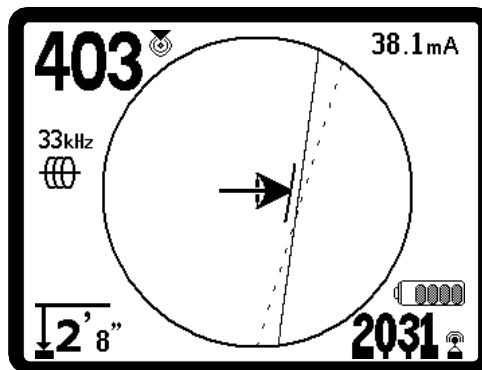
Figure 65: Screen Display with Distortion Line (Line Trace Mode)
