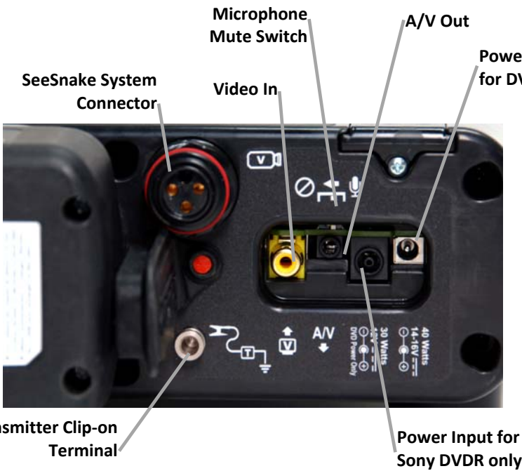
Figure 3: DVDPak Connections
